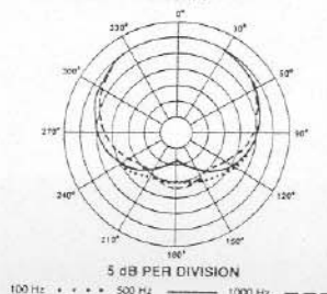
FIGURE 2 — Polars
