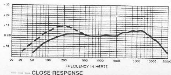
FIGURE 1 — Frequency Response
